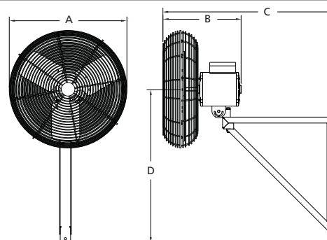
Figure 6 — 3PEH2 Dimensions
