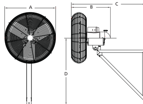
Figure 3 — 3PEG9 Dimensions
